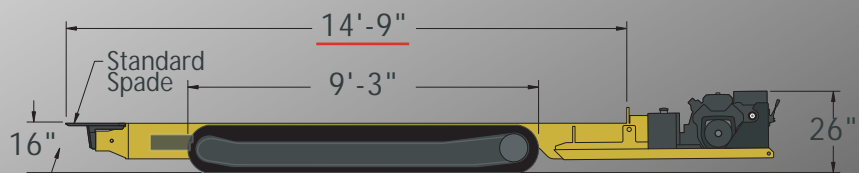
Lowered Dimensions
