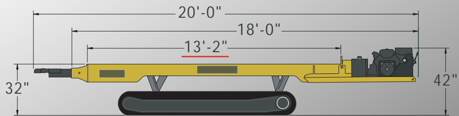
Raised Dimensions
