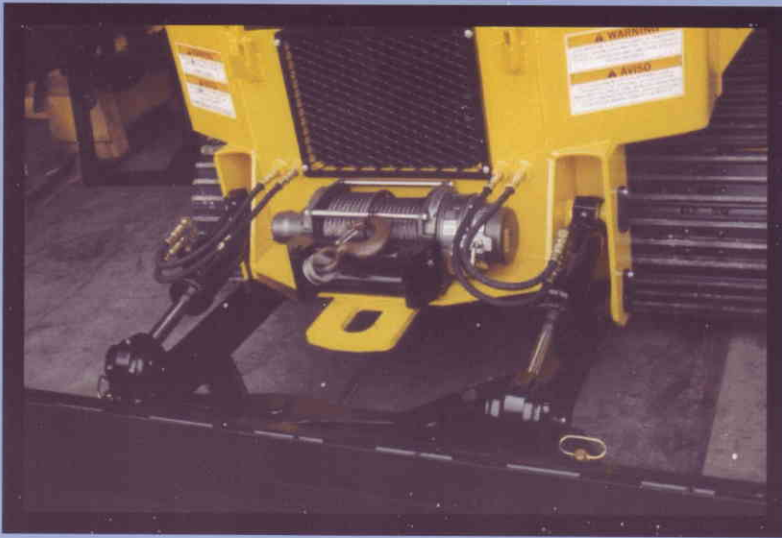
465 SHOWN WITH STANDARD 12,000 LB WINCH AND OPTIONAL DOZER BLADE ATTACHMENT
